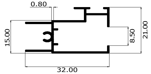
Section No. 2229 · Wt Range: 0.850-1.050 Kg/12ft
