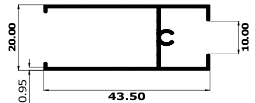
Section No. 2235 · Wt Range: 1.050-1.300 Kg/12ft
